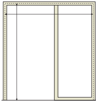
Door with Sidelight Nominal Door Width + Sidelight + 2" for each Mullion + 1 1/4" Jamb Height + 1"
