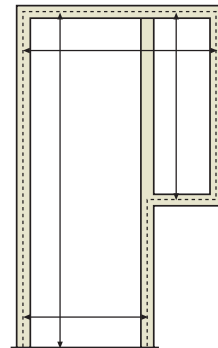
Door and Partial Sidelight UPPER: Nominal Door Width + Sidelight + 2" for each Mullion + 1 1/4" LOWER: Nominal Door Width + 1 1/4" Jamb Height + 1" Sidelight Height: Rabbet to Rabbet + 1 1/4"
