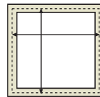
Borrowed Light Width = Rabbet to Rabbet + 1 1/4" Height = Rabbet to Rabbet + 1 1/4" Note: Actual glass size is smaller. Always measure frame before ordering glass
