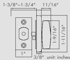
Privacy Deadbolt
