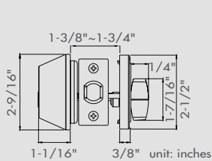
Single Deadbolt
